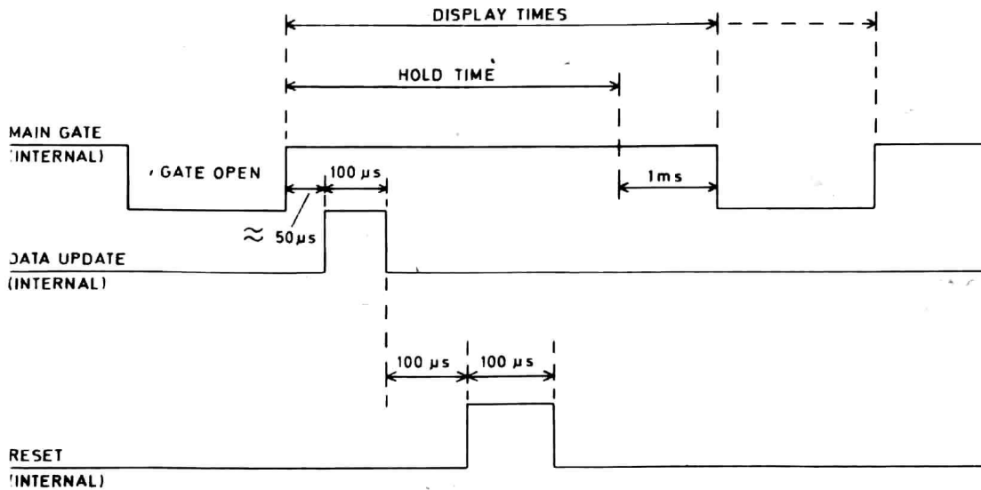
Control Sequence Diagram
