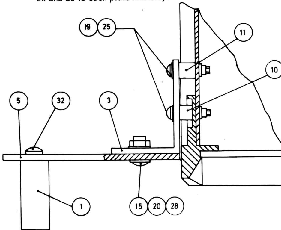
Plan View: Rack Mounting 11-1126 Fig.5
