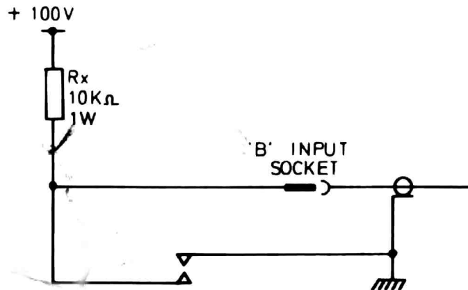
Contact Closure Supply Fig. 4
